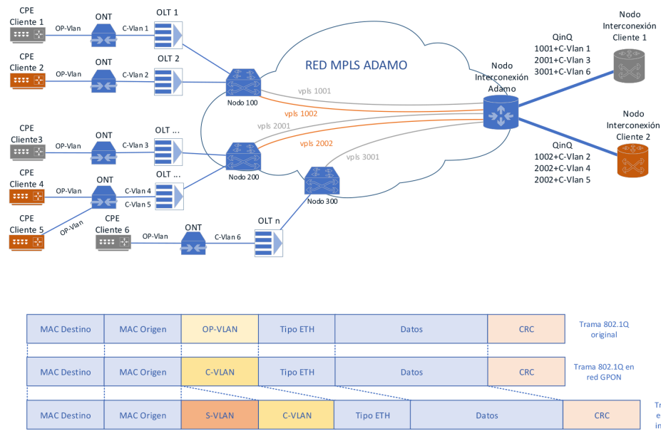
Figura 4 - BITSTREAM - modalidad Vlan per Service
